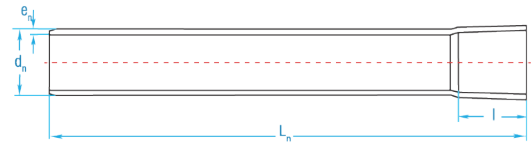
Ống có khớp nối dán keo/ Pipe with solvent cement socket
