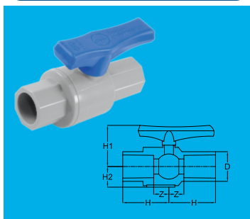
Van cầu / Ball valve
