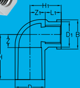
Co 90° ren ngoài Male thread 90° elbow
